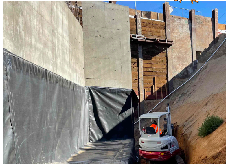
Looking east at progress on the Van Buren Boulevard bridge support system and the Jurupa Road retaining wall.
